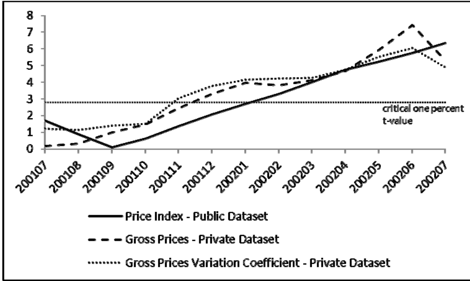
Figure 3: t-values for varying break points Source: Hüschelrath and Veith (2011)
