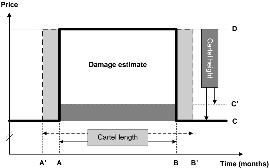
Figure 1: Cartel length, cartel height and the estimation of damages Source: own graph
