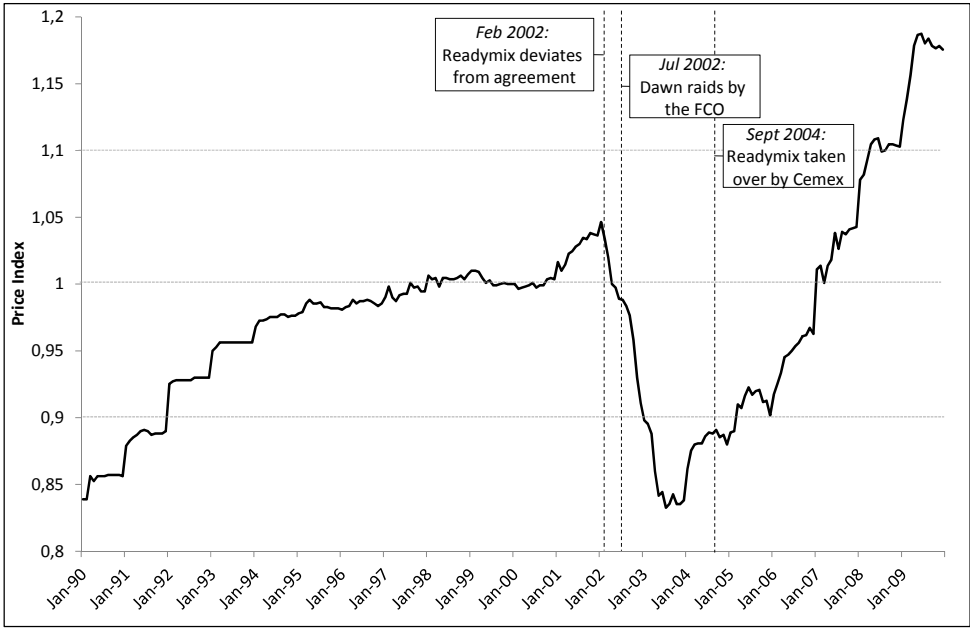
Figure 2: The public price index for cement from January 1990 to December 2009 Source: Own graph following Friederiszick and Röller (2010), p. 599
