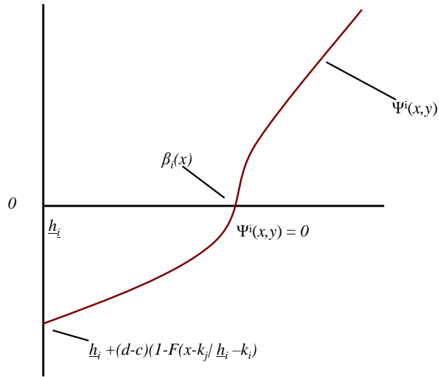
Figure 1: \Psi^i(x,y)
