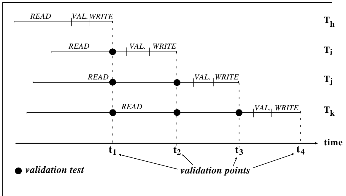
Figure 2: Snapshot validation
