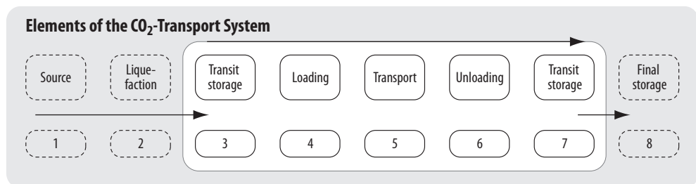
Figure 8: Elements of the CO 2 Transport System (source: Schlattmann 2006)
