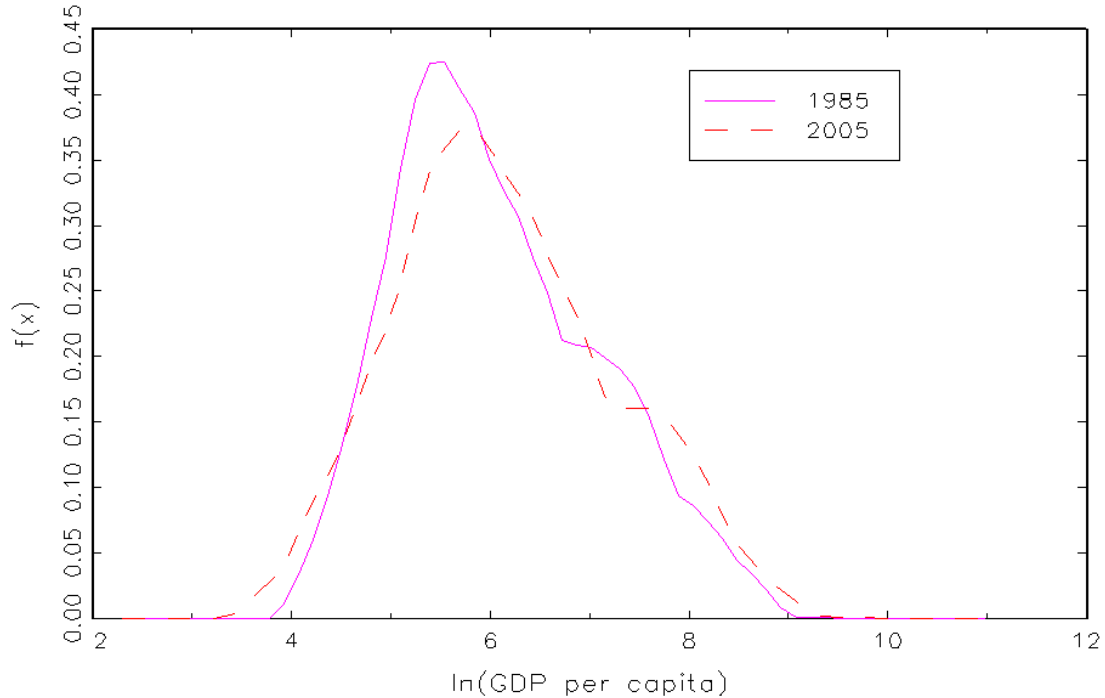
Africa GDP per capita distributions '85 – '05 (population weighted)
