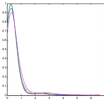
FIGURE 2: Estimates of the density of b^h(\mathbf{p}_t) = \left(\frac{1}{b_t} + \varepsilon_t^h\right)^{-1} (by period)
