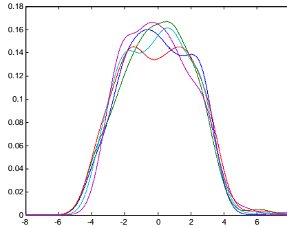
FIGURE 1: Estimates of the density of heterogeneity terms \varepsilon_t^h (by period)
