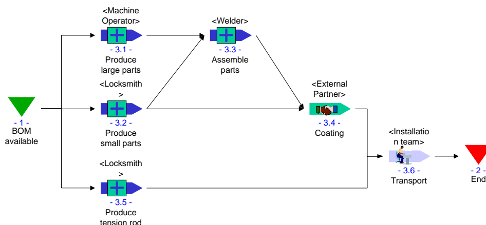
Figure 8: Sample production process 1
