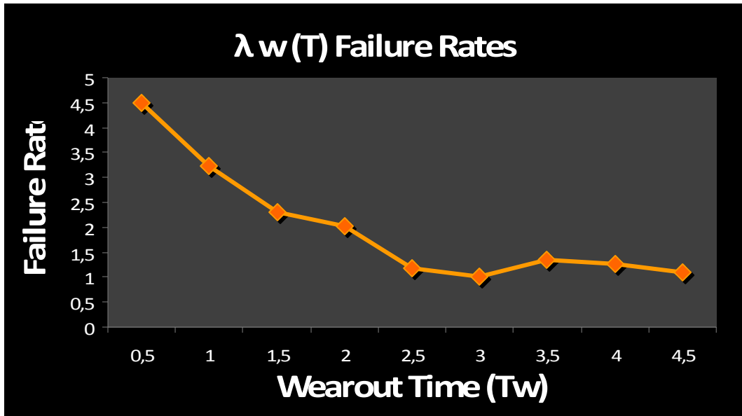
Figure 5: Failure rates in wear out period
