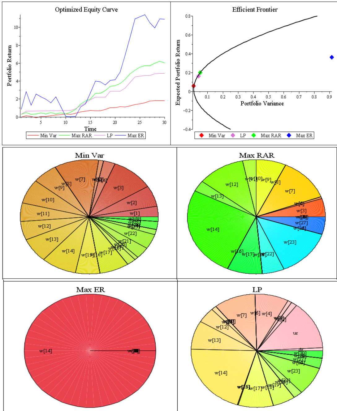
Figure 1: Simulated Data and Investment Strategies
