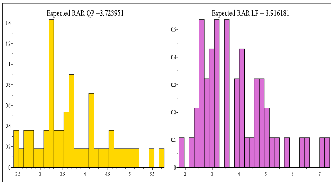
Figure 2: Simulated Data and Risk Adjusted Returns (RAR)
