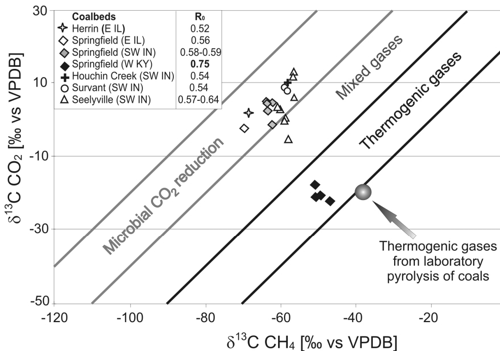
Fig. 2 Carbon isotopic signatures of methane and CO_2 in coalbed gases from the Illinois Basin. Coalbeds in the legend in stratigraphic sequence. Genetic ranges of gases and pyrolysis data after Smith and Pallasser 1996.
