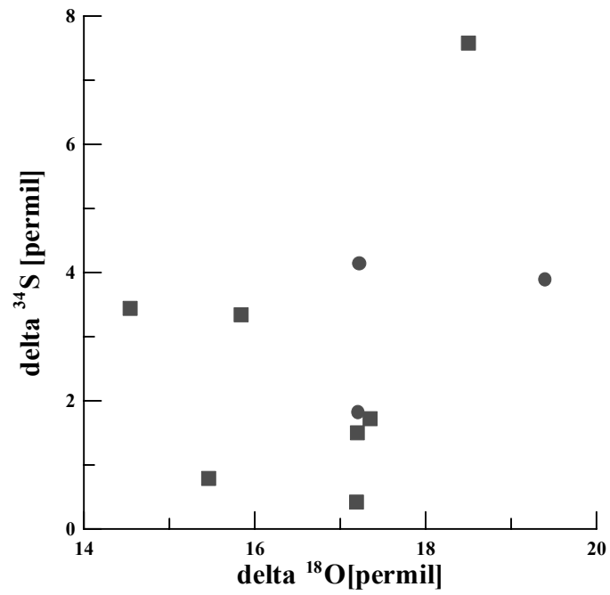
Fig. 4 A comparison of the isotope compositions of the mother solution (squares) and sulfate formed in recent summer precipitation (circles)
