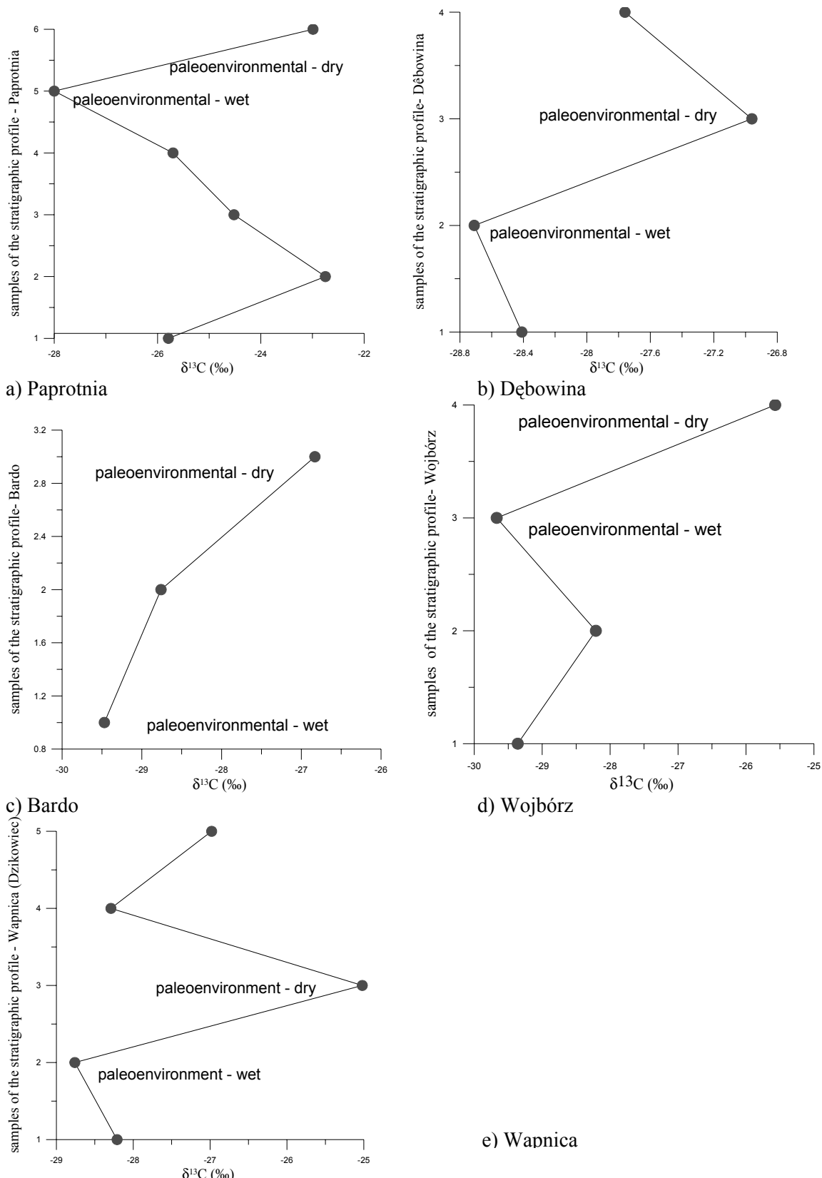
Fig. 1 Carbon isotope variations in Lower Carboniferous plants remains from Bardzkie terrestrial sedimentary series
