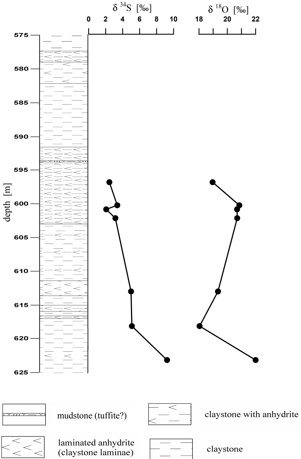
Fig. 3 Litologic section and isotope profiles of evaporitic sulfates in Woszczyce IG1 borehole
