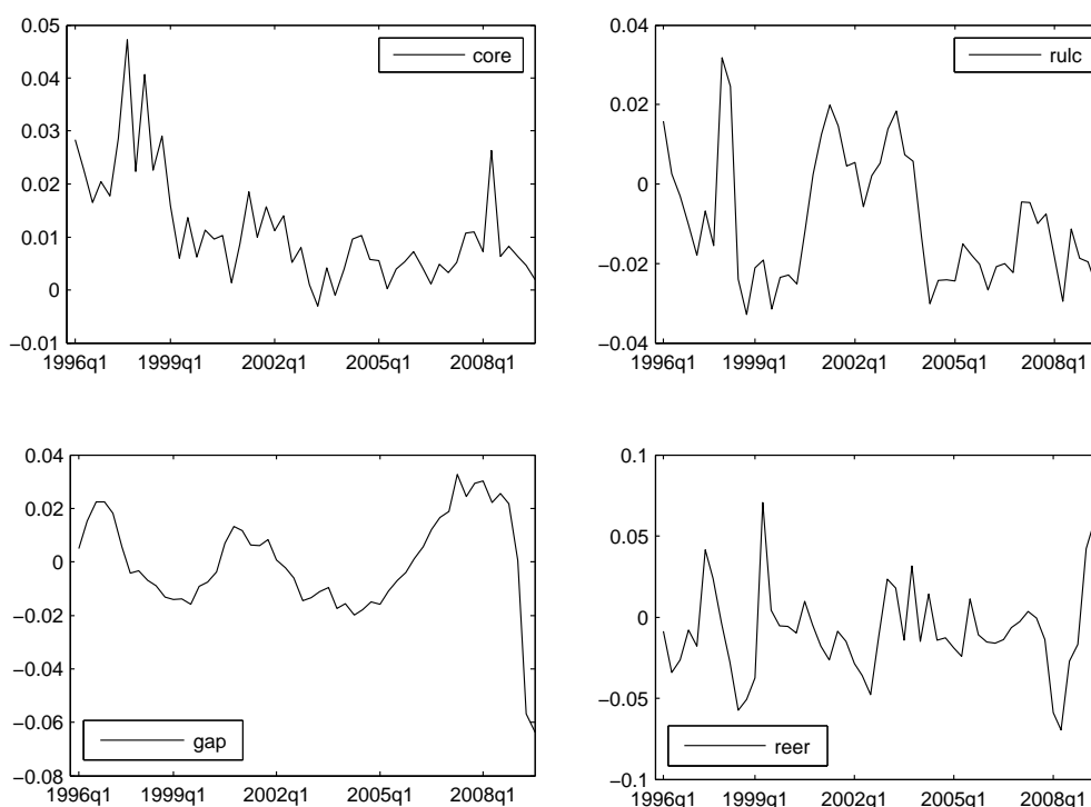
Figure 1: Selected time series for the Czech Republic, 1996-2009
