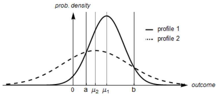
Fig. 1 Probability density functions of two alternative behaviors.
