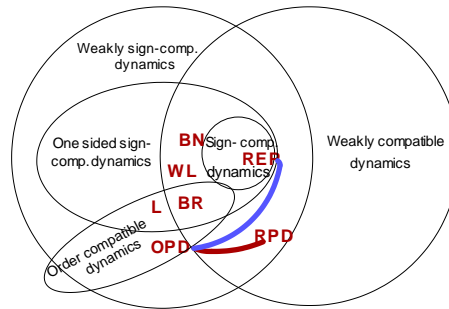
Figure 2: Relations between dynamics. The red line depicts barycentric ray-projection dynamics; the blue one q -deformed replicator dynamics, q \in [0, 1] .
