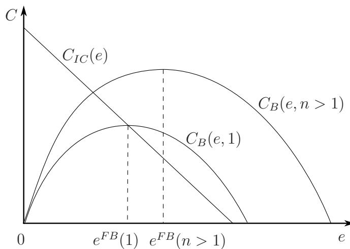
Figure 4: Uniqueness.
