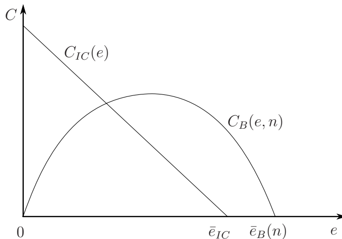
Figure 3: Existence.
