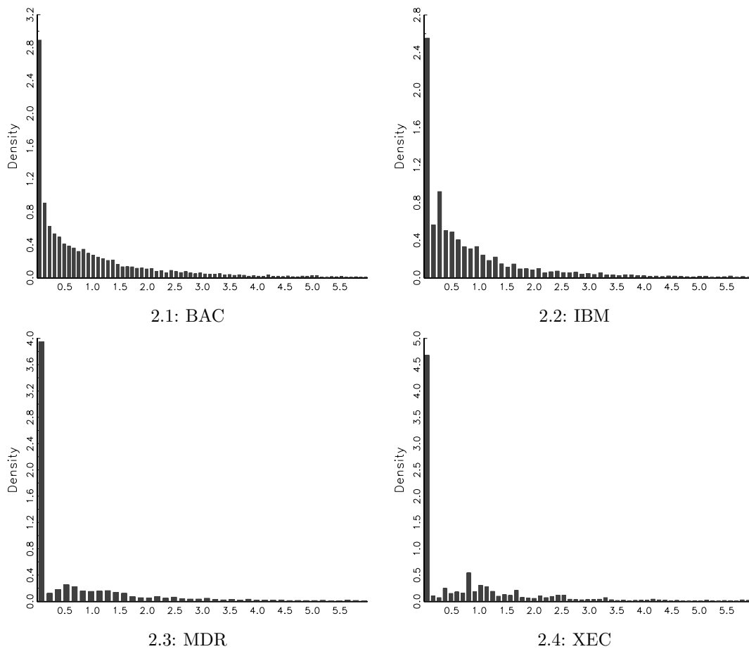
Figure 2: Sample Histograms of Deseasonalized Cumulated Volumes
