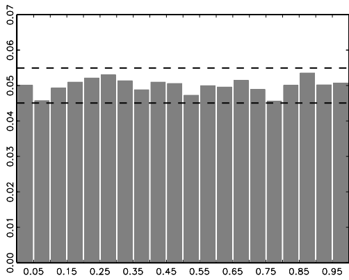
6.3: MDR
