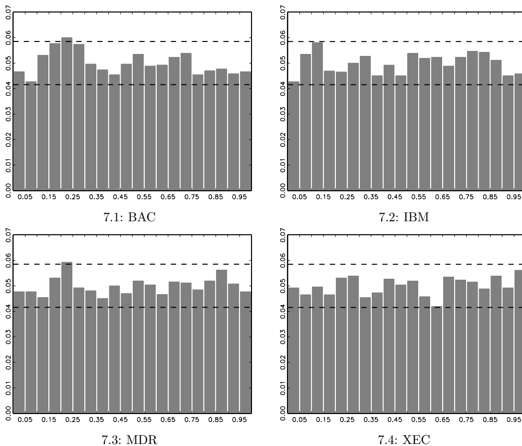
Figure 7: Histograms of Out-Of-Sample PIT Sequences
