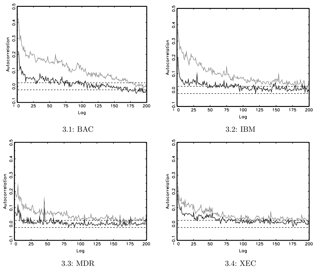
Figure 3: Sample Autocorrelograms
