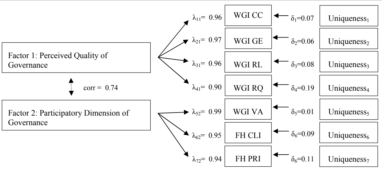
Figure 3: Loading Pattern CFA Model, Two Common Factor Model, Non-LIC Sample
