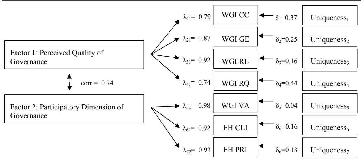
Figure 2: Loading Pattern CFA Model, Two Common Factor Model, LIC Sample
