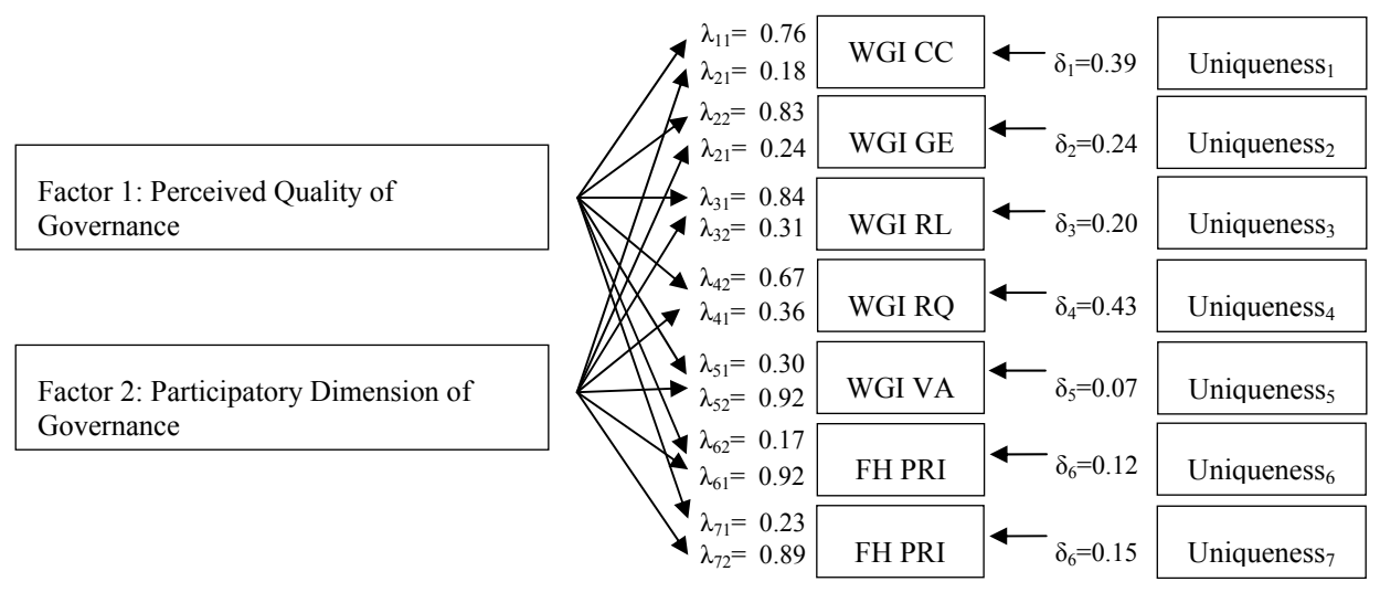
Figure 1: Loading Pattern, Orthogonal Two Common Factor Model, LIC Sample
