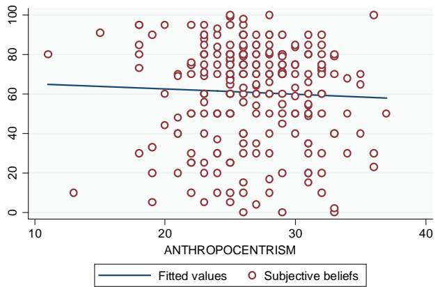
Fig. 4. Subjective beliefs VS Anthropocentrism
