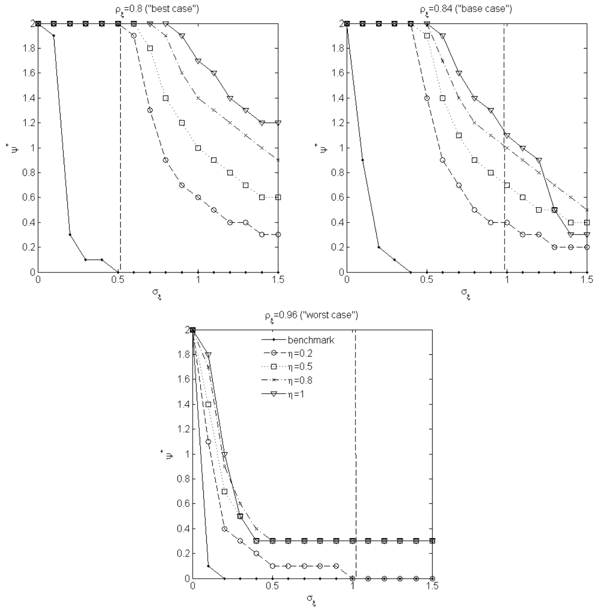
Figure 5: Optimal \psi given Output Gap Misspecification
