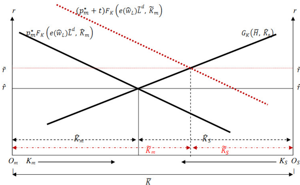
Figure 1 Graph of Equations (3) and (4), with t > 0
