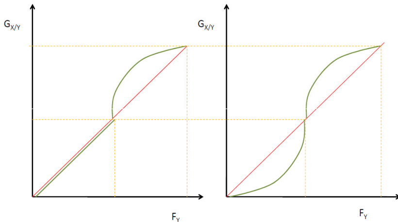
Figure 1: Left panel: the two CDFs overlap in part of their common support. Right panel: the two CDFs cross once
