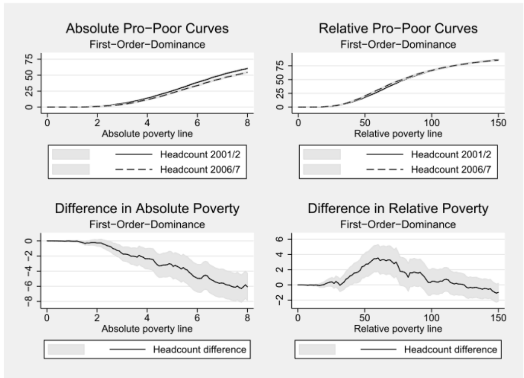
Figure A11: Unidimensional poverty dominance curves
