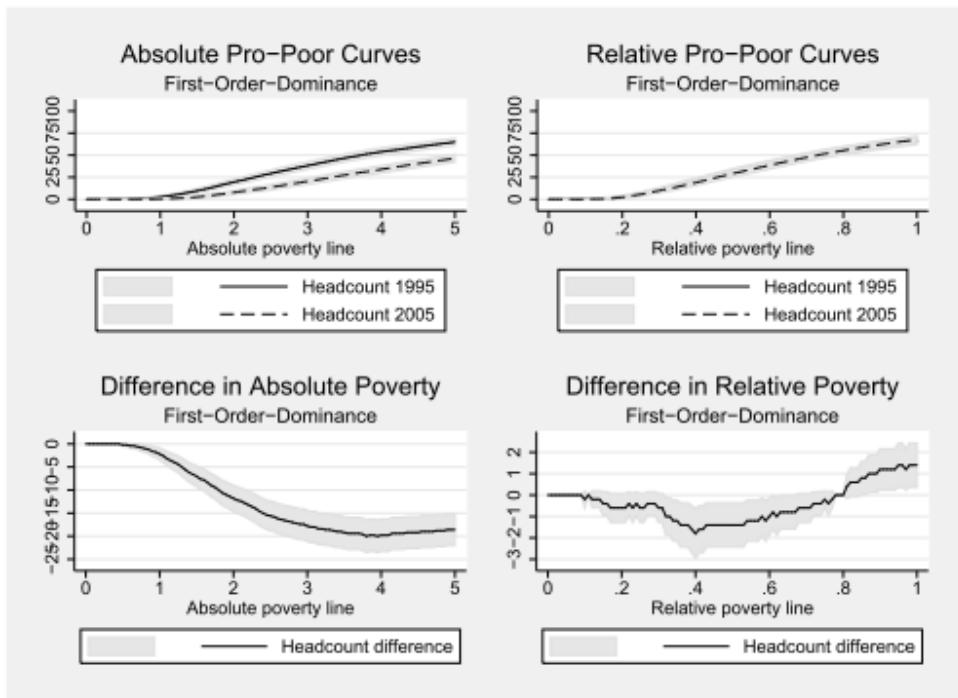
Figure A17: Unidimensional poverty dominance curves
