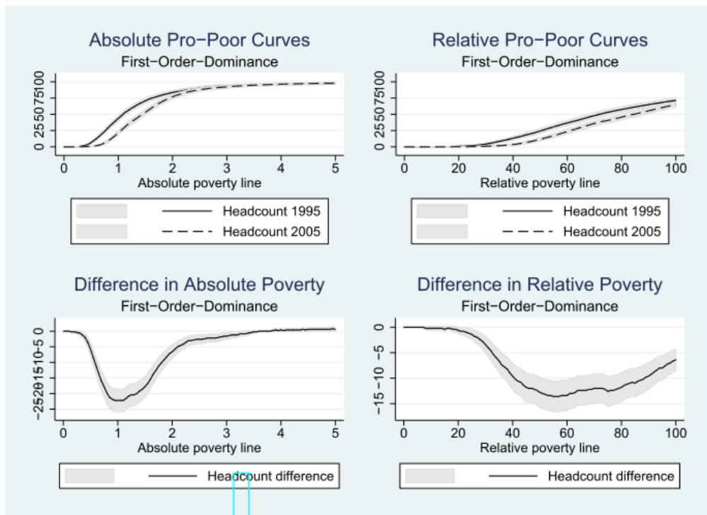
Figure A3: Unidimensional poverty dominance curves
