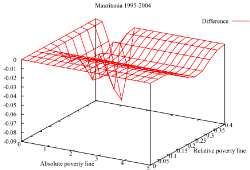
Figure A10: Bidimensional growth dominance curves
