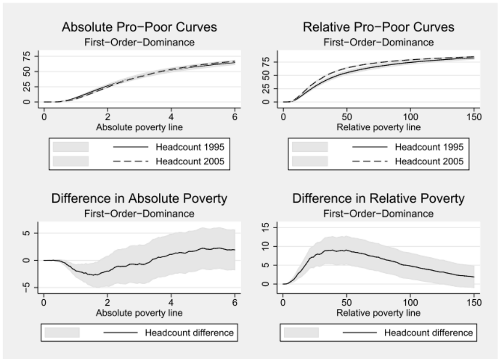
Figure A15: Unidimensional poverty dominance curves
