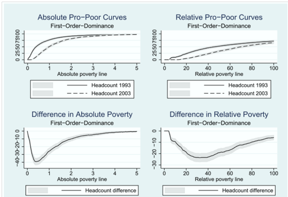
Figure A1 : Unidimensional poverty dominance curves
