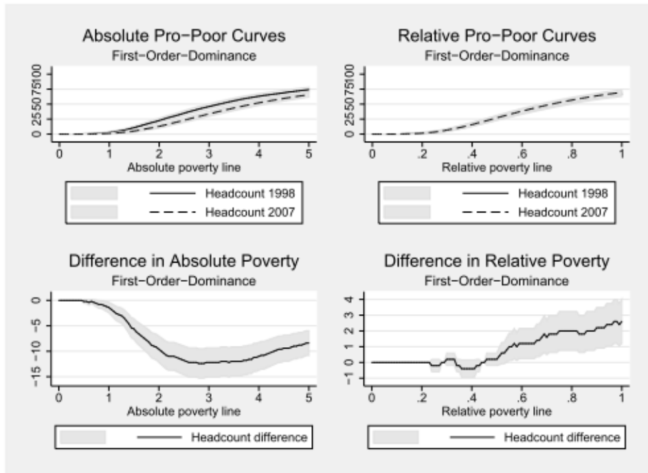
Figure A13: Unidimensional poverty dominance curves
