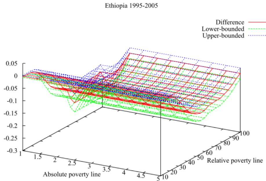
Figure A4: Bidimensional growth dominance curves
