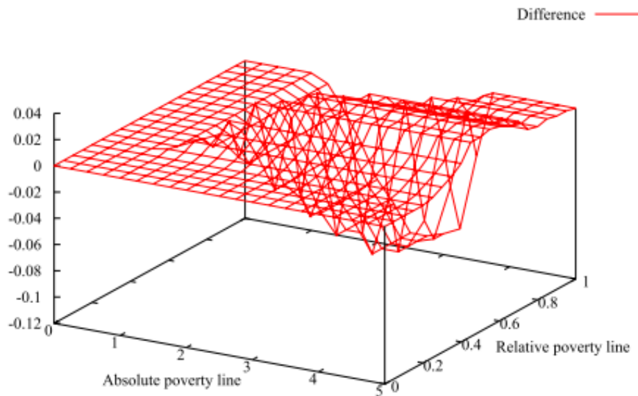
Figure A8: Bidimensional growth dominance curves
