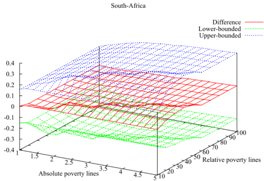
Figure A16: Bidimensional growth dominance curves
