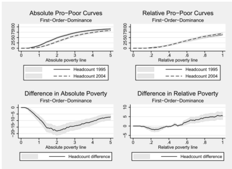
Figure A9: Unidimensional poverty dominance curves
