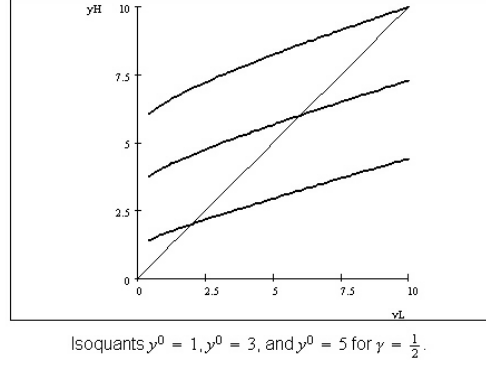
Figure 7: Isoquants y^0 = 1 , y^0 = 3 , and y^0 = 5 for (\alpha, \beta, \gamma, y^L) = (0, \beta, \frac{1}{2}, y^L) .
