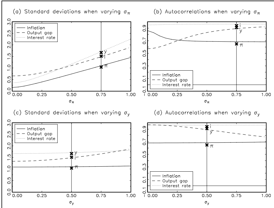
Figure 5: Varying the standard deviation of shocks from the baseline configuration
