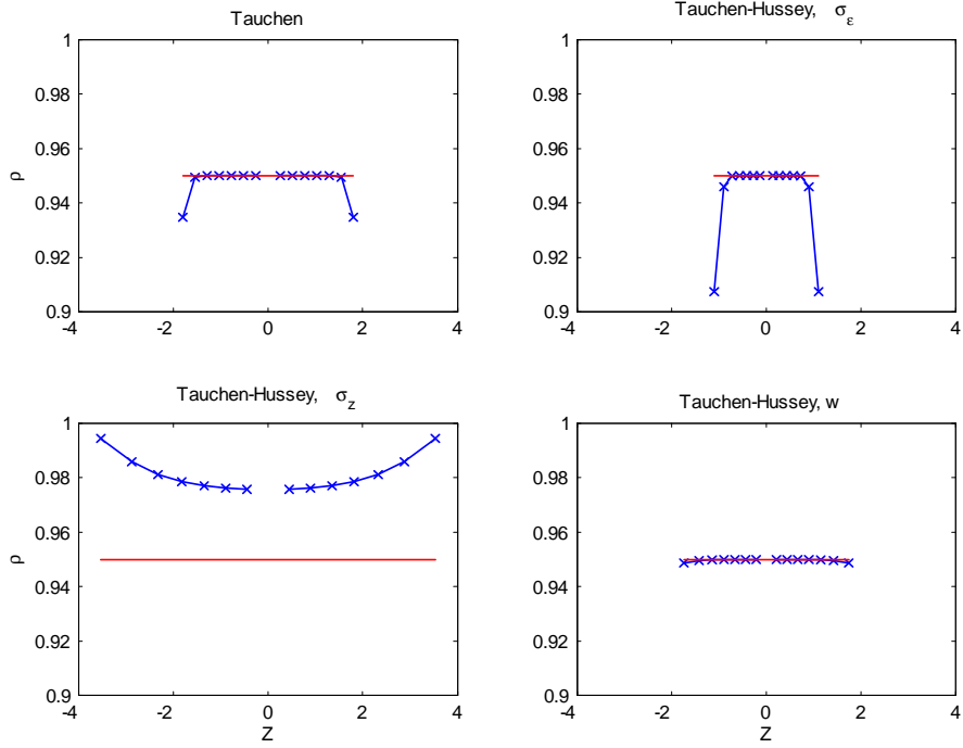
Figure 1: Approximation of the HSZ process with 15 nodes, true (red) \rho and \rho conditional on node (blue, marked)
