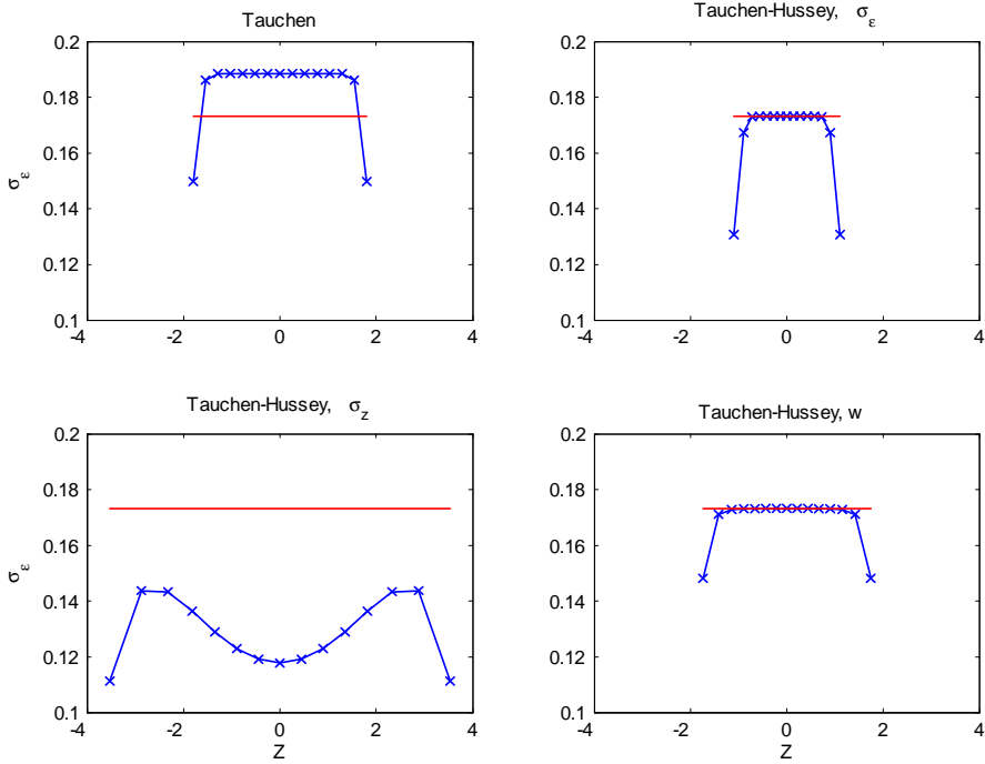
Figure 2: Approximation of the HSZ process with 15 nodes, true (red) \sigma_\epsilon and \sigma_\epsilon conditional on node (blue, marked)
