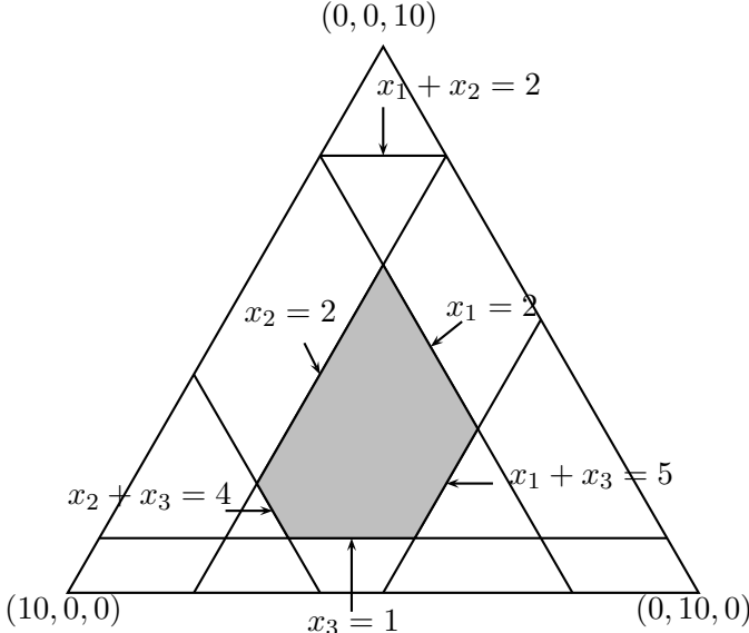
Fig. 1. Core of the game v
