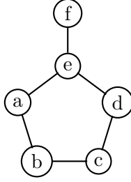
Fig. 2. Neighboring extreme points of \text{Core}(v) .
