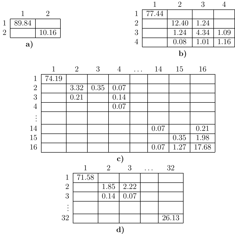
Figure 7: Distribution of the sizes of minimal sCURB sets a) in random 2 \times 2 games, b) in random 4 \times 4 games, c) in random 16 \times 16 games, d) in random 32 \times 32 games
