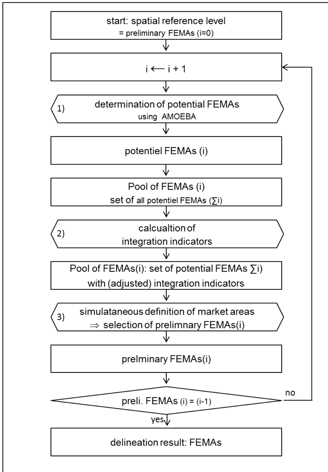
Figure 1: Overview delineation procedure
