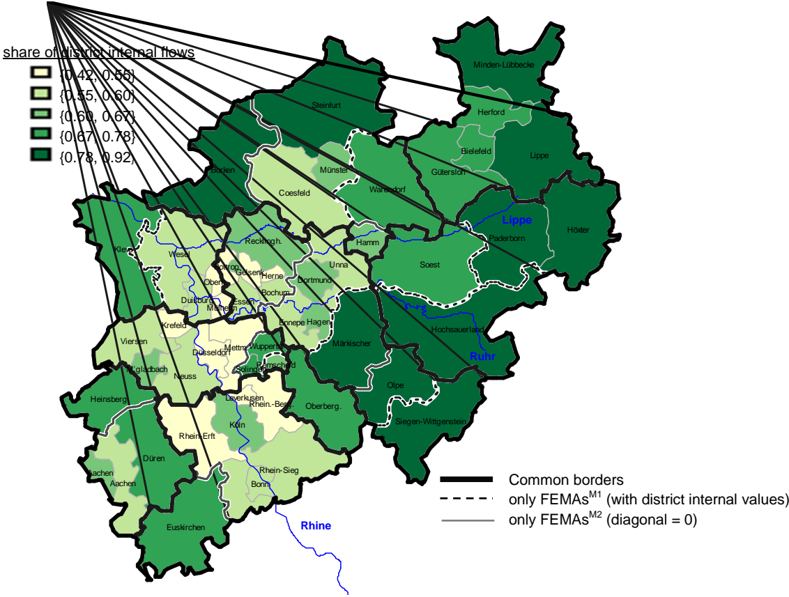
Figure 3: Delineation results for NRW illustrate together with shares of district internal flows
