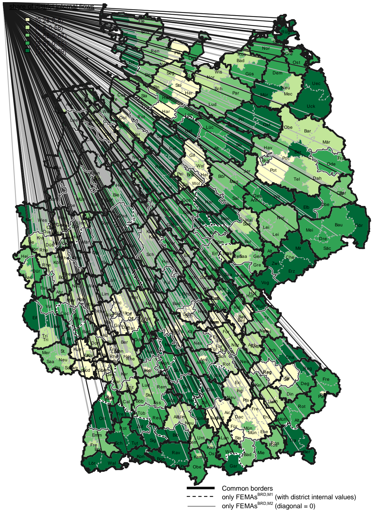
Figure 6: Delineation results for Germany 43
