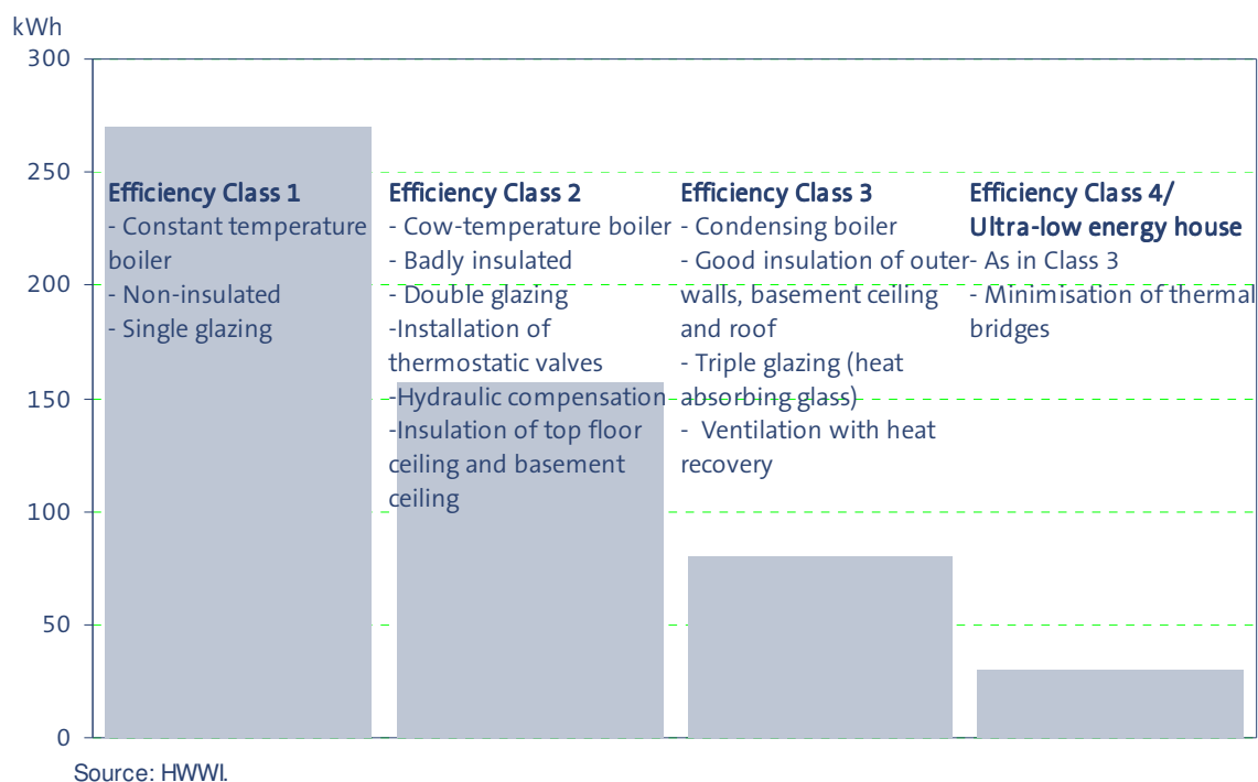
Figure 2.3: Efficiency Classes of Heating Energy Sources Using Oil as an Example
