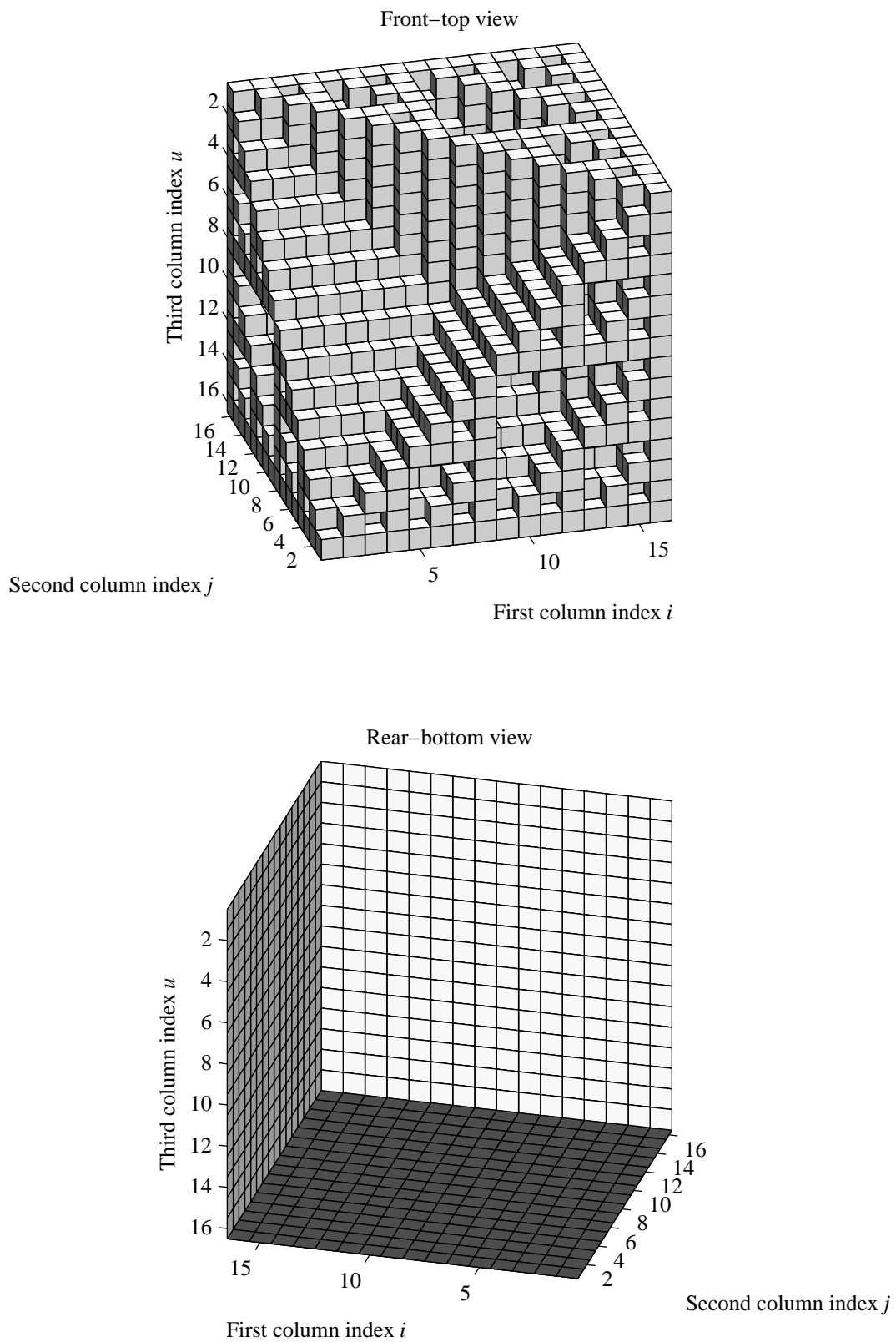
Figure 4: Triplets of 4-columns with a perfect column pair (union of three Sierpinski cylinders)
