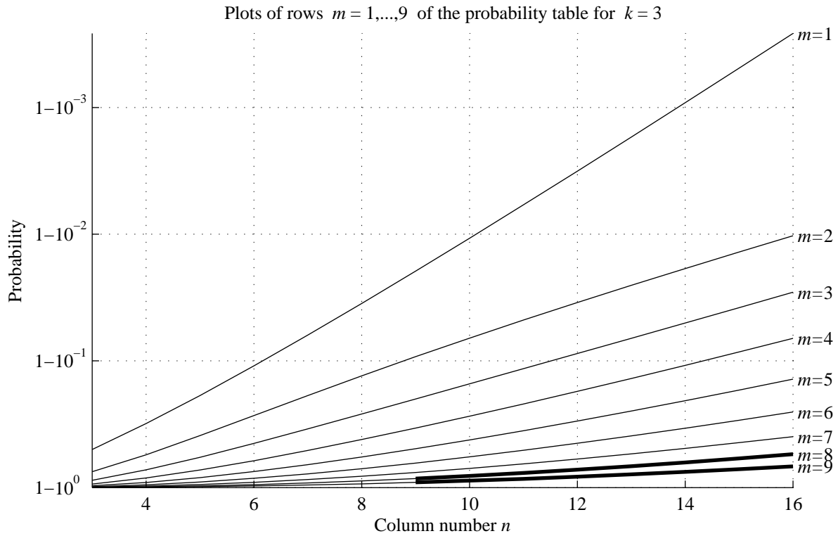
Figure 11: Plots of the logarithmically scaled first columns and first rows of Table 25 of probabilities of perfect column triplets ( k = 3, i = 0 ) with the interpolated segments shown by thick curves
