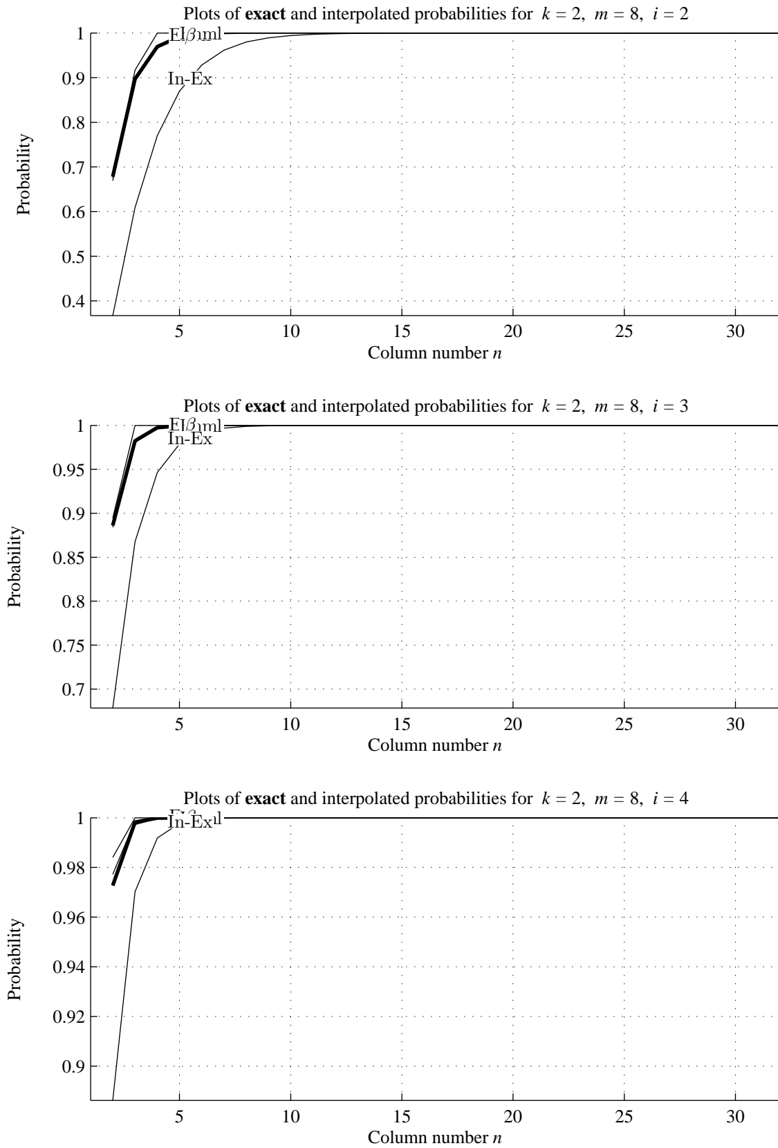
Figure 13: Plots of interpolated probabilities of i -imperfect column pairs ( k = 2 ) in Bernoulli ( m \times n )-matrices. The interpolation is made by exponential, binomial, and beta curve fit and with the Inclusion-Exclusion formula and denoted respectively as Expn, Bnml, \beta , and In-Ex. The exact probabilities, if known, are shown by thick segments.
