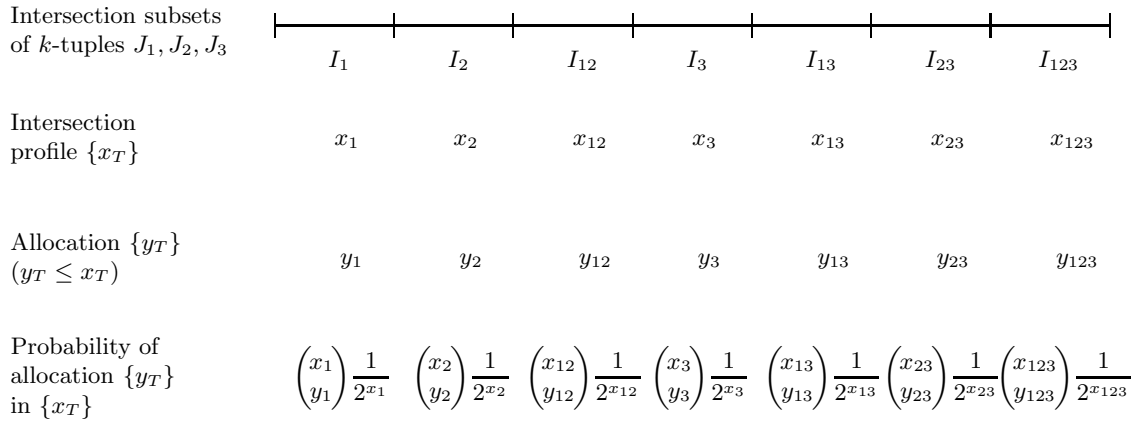
Figure 7: Intersection profile of three k -tuples, allocation, and its probability
