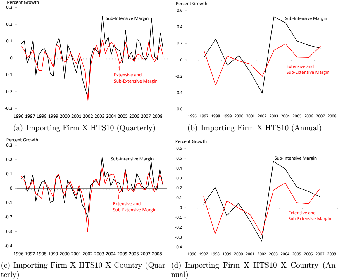
Figure 5: Sub-Extensive Margin
