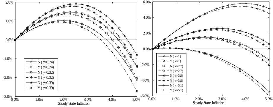
Figure 3: Sensitivity with respect to guilt parameters
