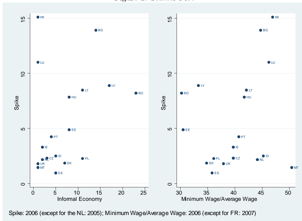
Figure 1: Scatter Plot
