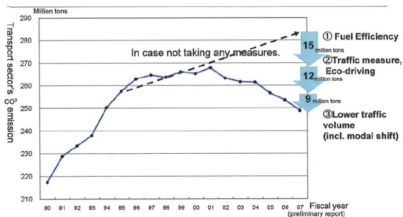
Figure 8: CO 2 Emissions from the Transport Sector (1990–2007)
