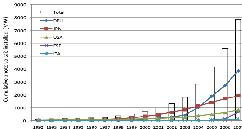
Figure 4: Cumulative Photovoltaics Installed in Top 5 Countries of 19 OECD Member Countries
