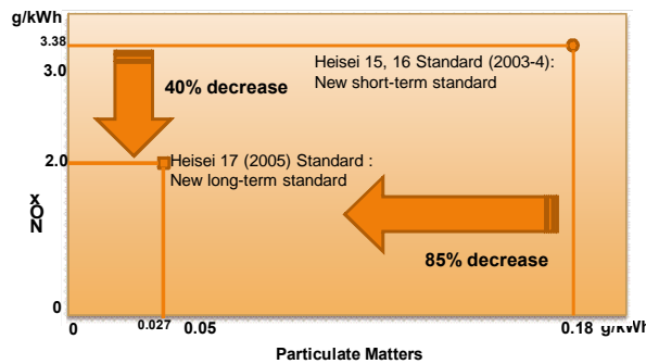
Figure B: Diesel Vehicle’s Emission Standard in the Heisei 17 Emission Standard
