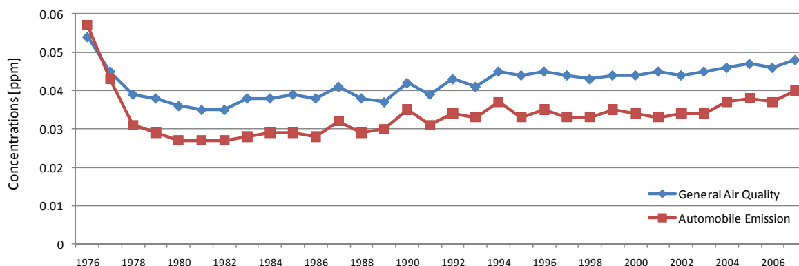
Figure 11: Annual Averages of Detected Day Time One-Hour Maximum Concentrations of Photochemical Oxidants at Monitoring Stations for General Air Quality and Automobile Emissions
