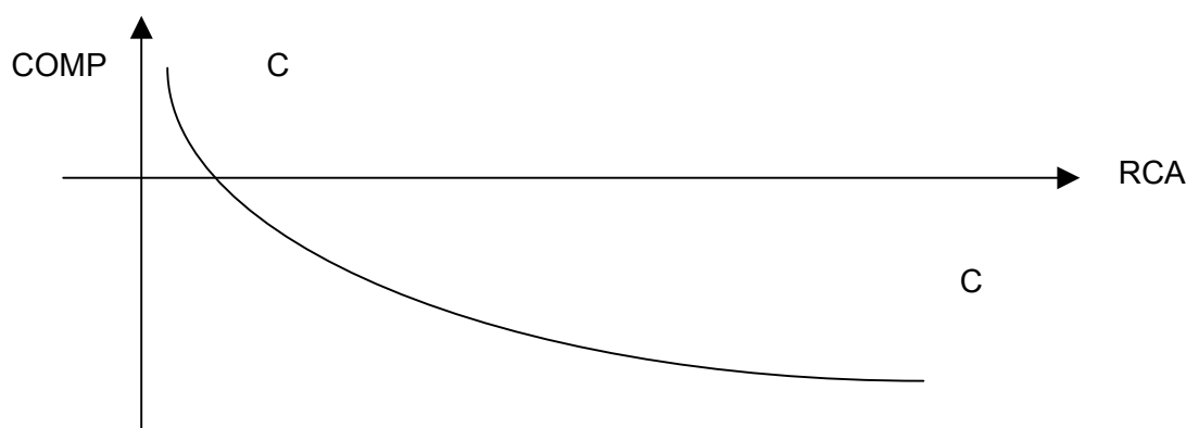
Fig 2. Illustration of RCA and competitiveness change
