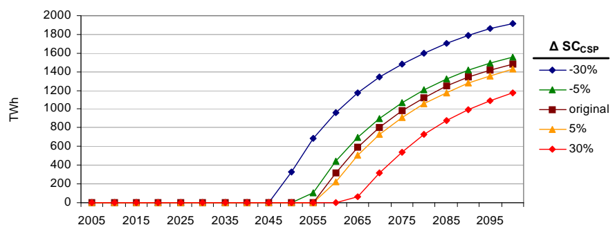
EU-Mena trade of SG-CSP Electricity
