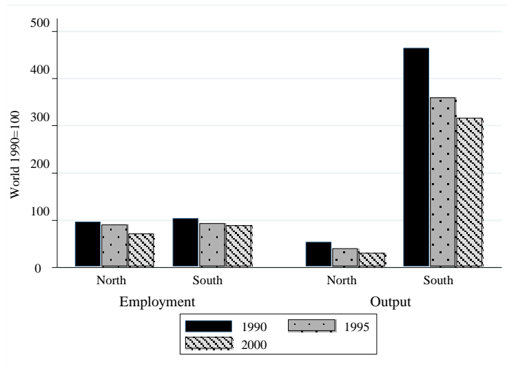
Figure 1: SO 2 Emission Intensities for North and South
