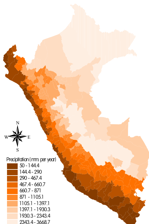
Map 3: Precipitation
