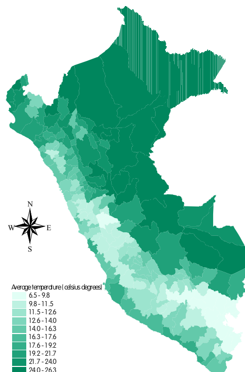
Map 4: Temperature
