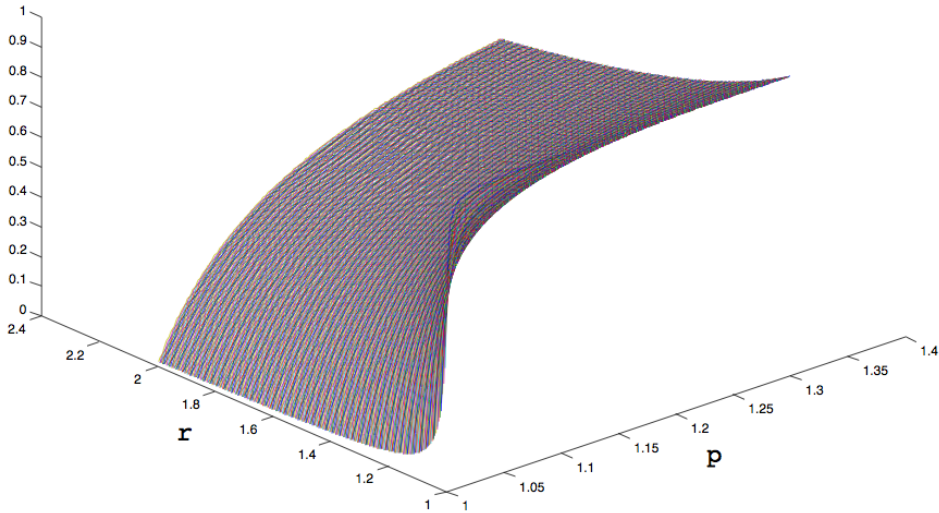
Figure 1: Graph of \gamma^* as a function of p \equiv \frac{\pi_1}{\pi_0} and r \equiv \frac{s}{\delta} .
