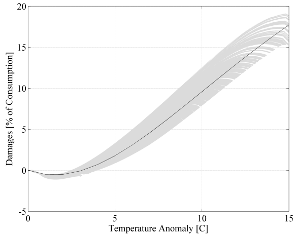
Figure 9: FUND Output and Approximate Damage Function
