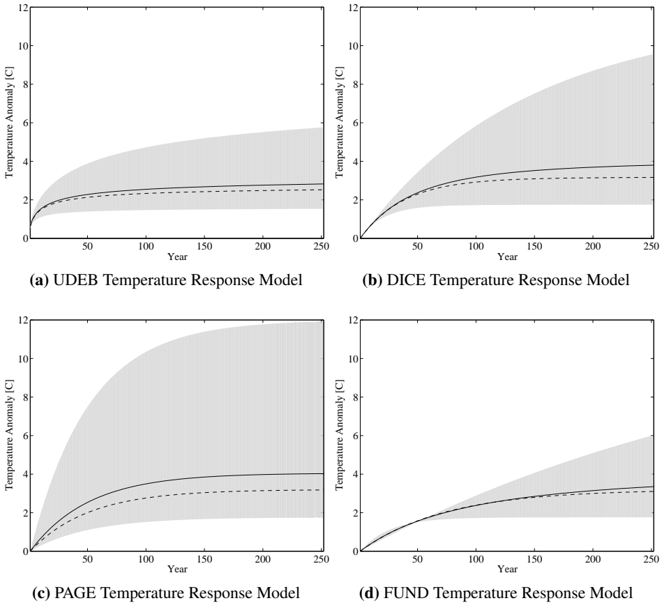
Figure 3: Temperature Response to a Sustained Doubling of CO 2
