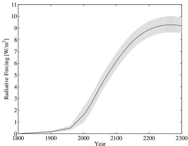
Figure 8: Radiative Forcing Scenario
