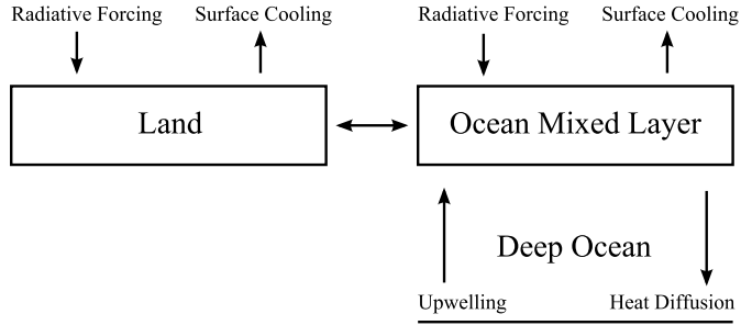
Figure 2: Simple Climate Model
