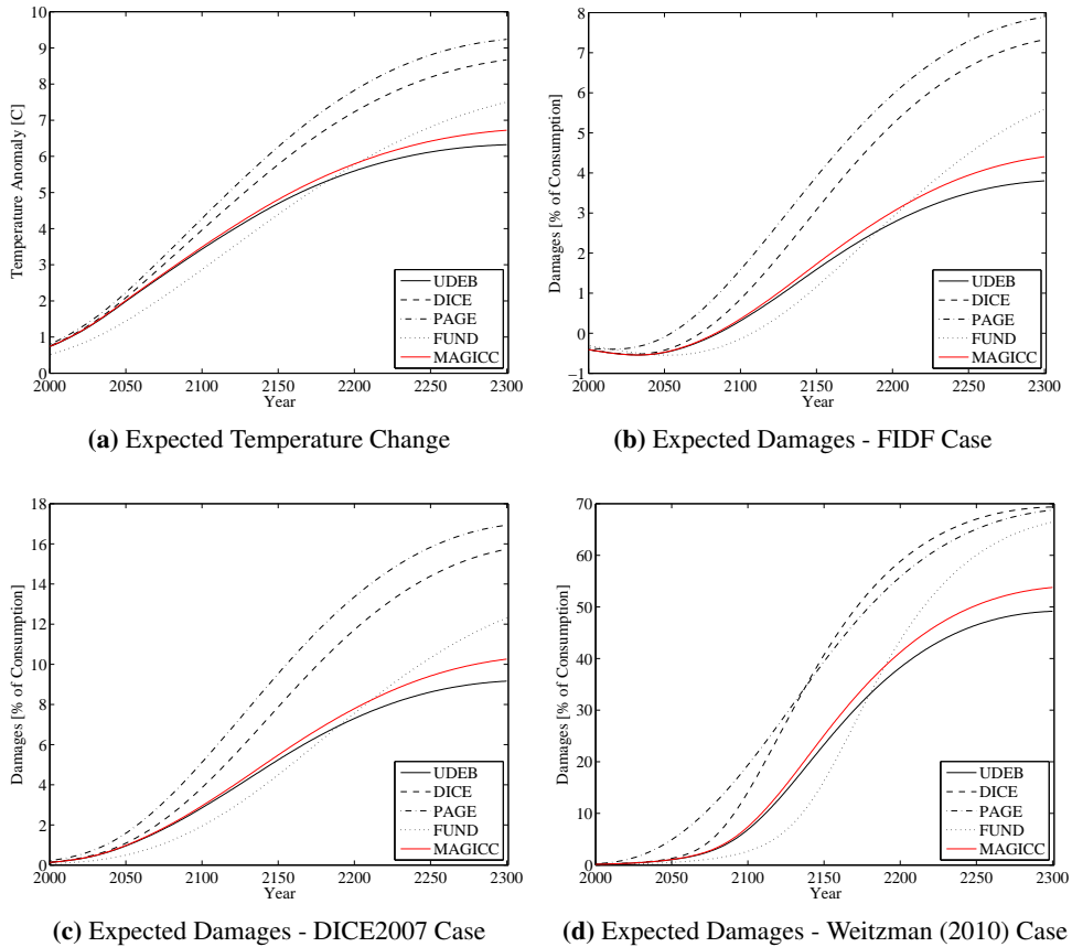
Figure 5: Mean Temperature Change and Damage Estimates
