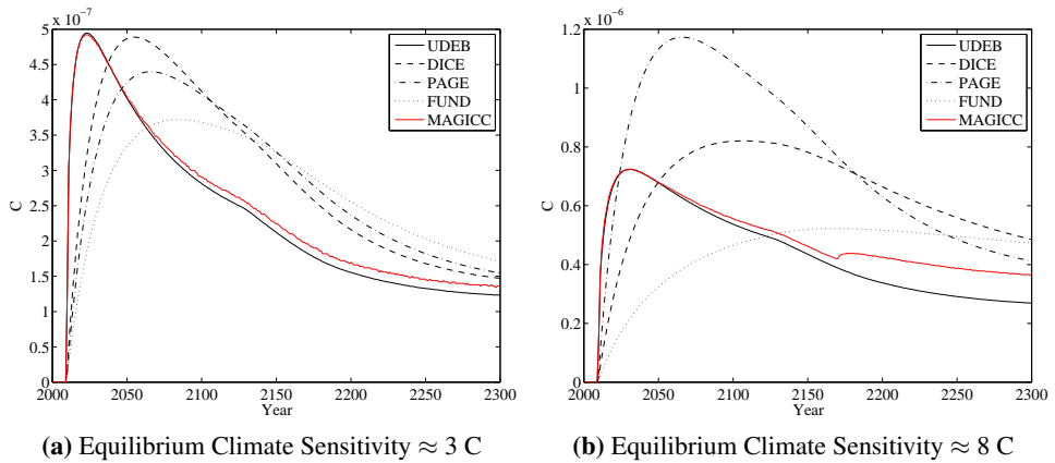
Figure 6: Temperature Perturbation From Additional Tonne of CO 2 Emissions in 2010
