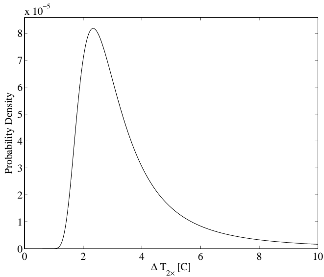
Figure 1: Probability Density Function for Equilibrium Climate Sensitivity
