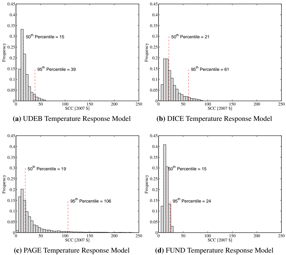
Figure 7: SCC Histograms Using DICE Damage Function and Constant 3% Discount Rate
