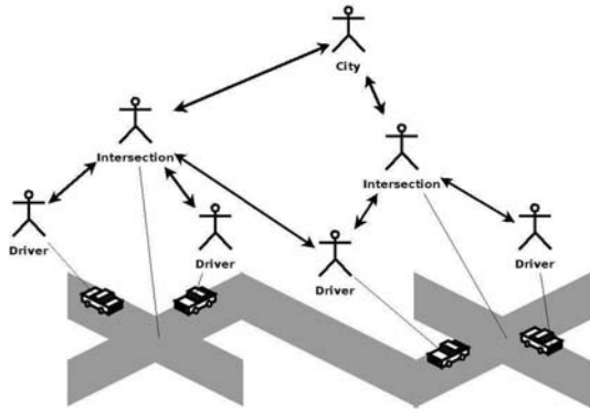
Figure 1: Overview of the multi-agent system
