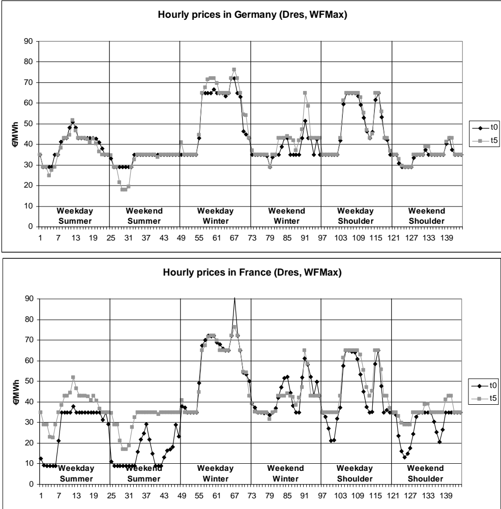
Figure 10: Hourly prices in France and Germany before and after extension ( DRes , WfMax )
