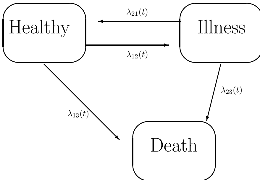
Figure 1: Illness-death model
