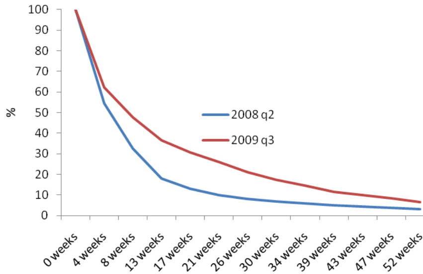
Figure 12: Survival function unemployment including activation. 2008.2 and 2009.3
