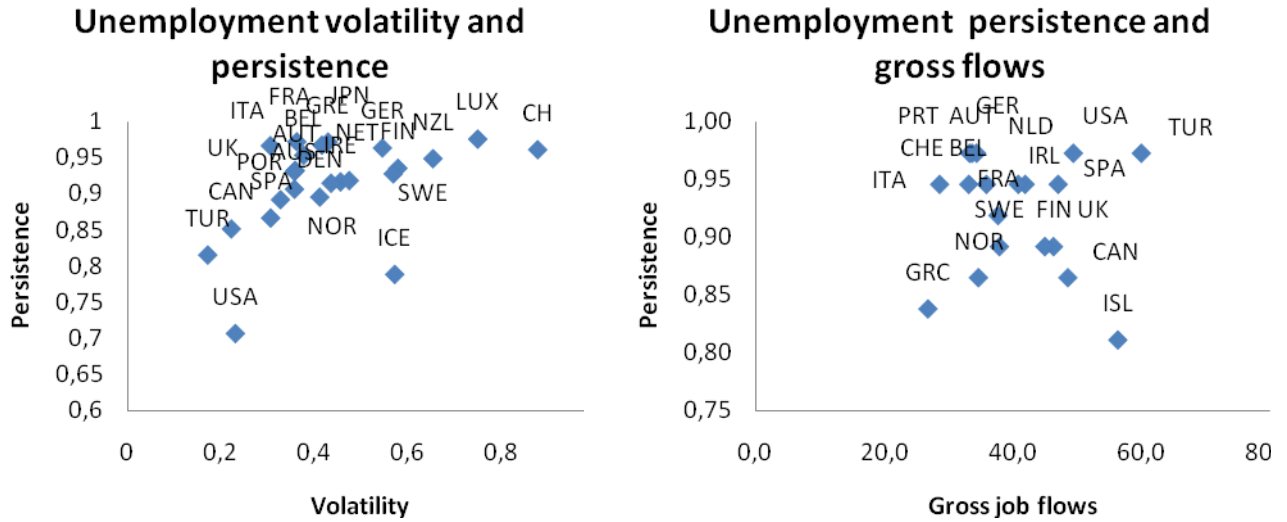
Figure 17: Labour market volatility and persistence
