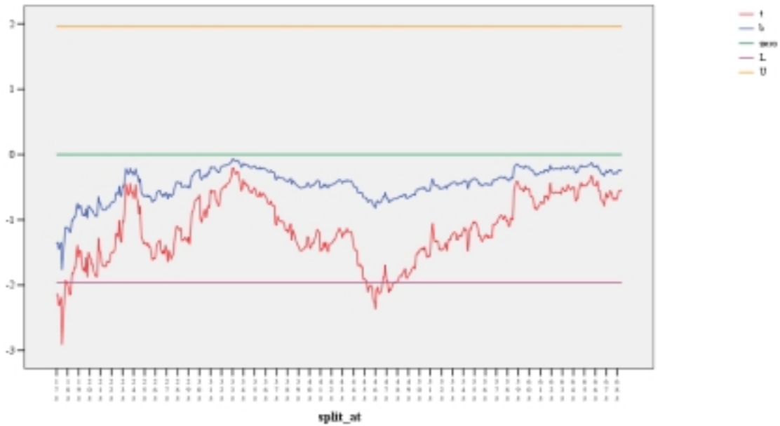
Graph 4: Threshold variable: \delta_{i,t}(Y/L) ; sample = observations 145–820, point estimate and t-statistics for \beta_5 ; traditional 95% confidence interval
