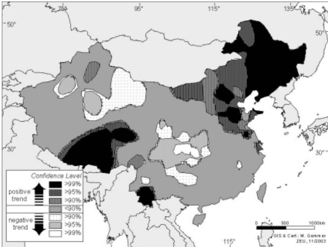
Figure 21: Mann-Kendall Temperature Trend Test March 1951-2002
