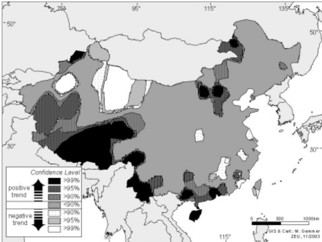
Figure 26: Mann-Kendall Temperature Trend Test August 1951-2002
