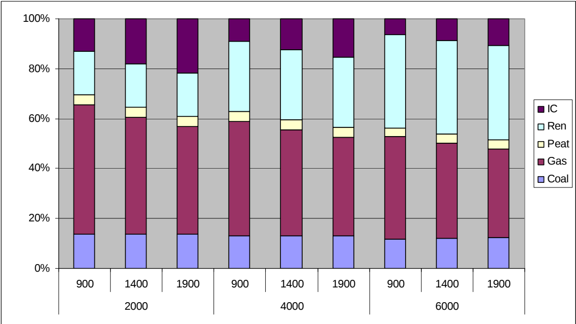
Figure 3. CCGT fuel shares in demand, medium fuel prices.
