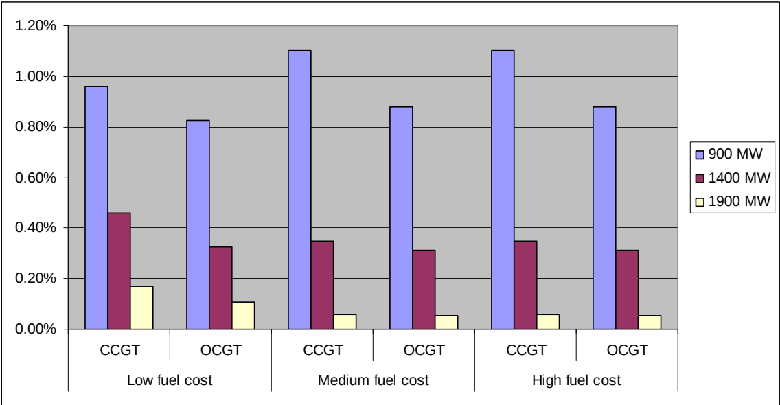
Figure 2. Wind Curtailment, 6000MW wind, CCGT and OCGT
