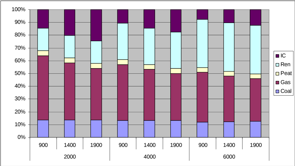
Figure A.1. OCGT fuel shares in demand, medium fuel prices.
