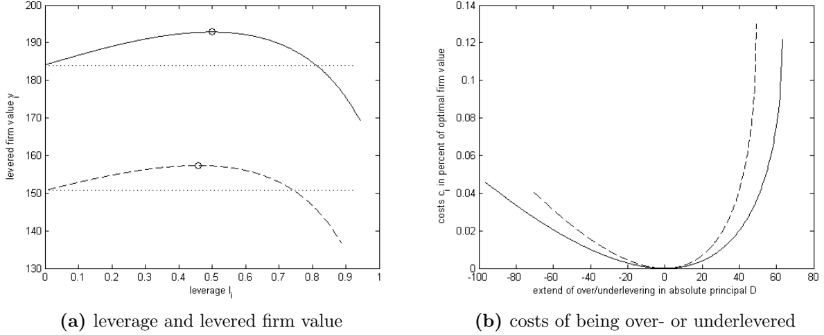
Figure 2: Panel (a) shows the levered firm value in dependence of chosen leverage. All parameters correspond to the values in table 1. The solid line is the levered firm value in a expansion ( i = 1 ), the dashed line in a recession ( i = 2 ). The upper dotted line is the unlevered firm value in an expansion and the lower dotted line the unlevered firm value in a recession. The optimal levered firm values are marked with a circle. Panel (b) shows the costs of being over- or underlevered. The x-axis is the deviation D of the chosen principal from the optimal leverage in the corresponding state. The cost of being over- or underlevered c_i(D) are measured as difference between the optimal and the chosen levered firm value in percent. The solid lines are the cost in an expansion and the dashed line in a recession.
