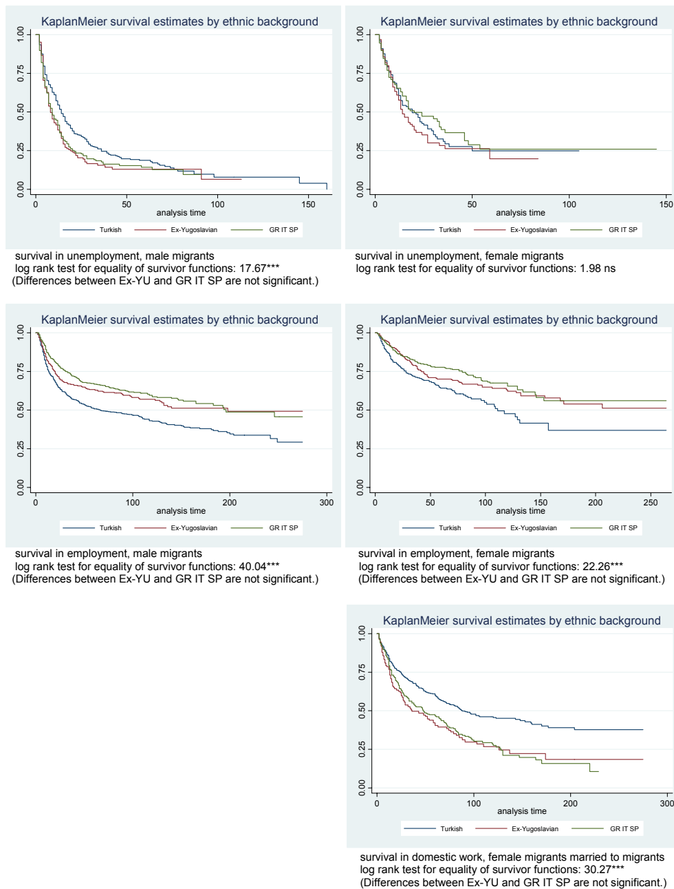
Figure 2: Survivor functions
