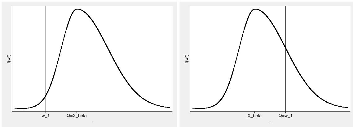
Fig. 3: Density of w^* = X\beta + \epsilon_i for X\beta > w_1 and X\beta < w_1
