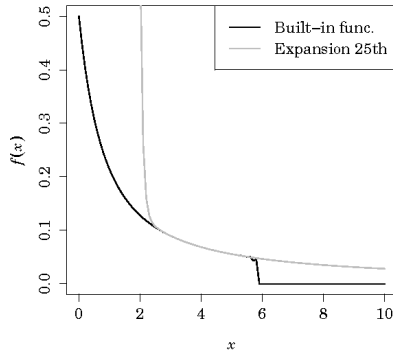
(a) Black line represents f(x) in (21) computed using a built-in error function; Gray line represents the same function f(x) , but it is computed using an equation obtained from asymptotic expansion equation (up to x to the 25th power).
