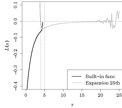
(b) Black line represents L(x) in (15) computed using a built-in error function; Gray line represents the same function L(x) , but it is computed using an equation obtained from asymptotic expansion equation (up to x to the 25th power).
